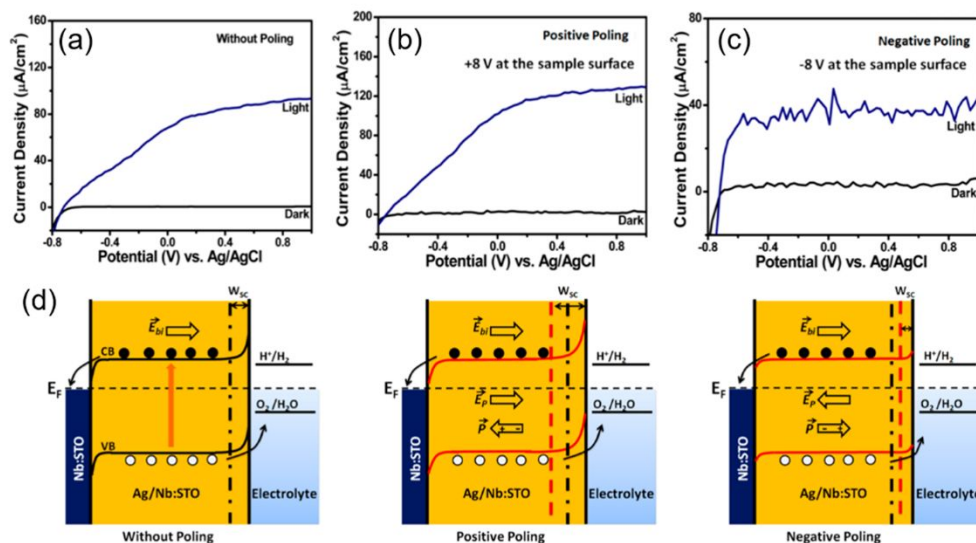
Fig. 9. Ag/Nb-doped STO nanoporous film for PEV water splitting. J-V curves of (a) unpoled, (b) positively poled, and (c) negatively poled Ag/Nb-doped STO thin film photoanodes under \sim 100 \text{ mW/cm}^2 illumination in 0.5 M NaOH solution. (d) Schematic band diagrams of ferroelectric Ag/Nb-doped STO photoanode interfacing with electrolyte without poling (left), and with positive (middle) and negative (right) poling, respectively. Reprinted with permission from ref 105. Copyright 2019 ACS.
