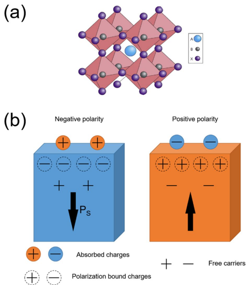
Fig. 2. (a) The extended network structure of cubic perovskite linking through the corner-shared octahedral. Reprinted with permission from ref 81. Copyright 2014 Nature Publishing Groups. (b) A schematic diagram of charges absorption near the polar surface. The direction of the arrow is parallel with the spontaneous polarization at the surface. Modified with permission from ref 86. Copyright IOP Science.
