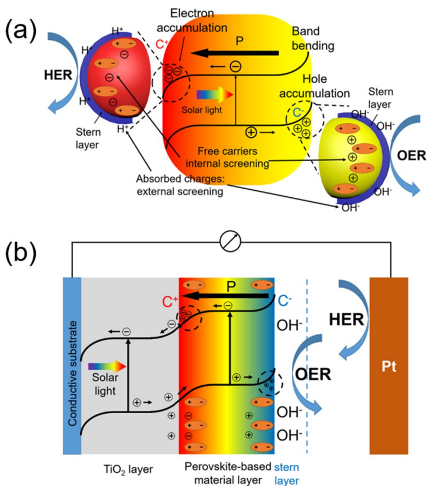
Fig. 3. (a) Schematic diagram of PC water splitting by internal and external screening due to the polarization in ferroelectric materials. (b) Schematic diagram of PEC water splitting by internal and external screening due to the polarization in perovskite-based material.
