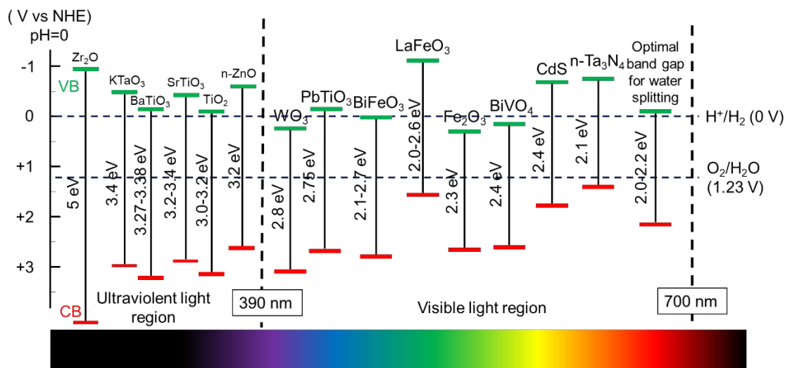
Fig. 2 Band edge positions of different semiconductors using in water splitting and their corresponding light absorption regions.
