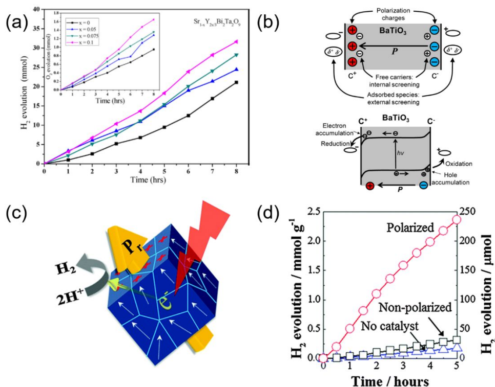
Fig. 10. Ferroelectric-enhanced photocatalytic water splitting. (a) The amount of H 2 /O 2 evolution using CH 3 OH/AgNO 3 scavengers for the 0.2 g of Sr 1-x Y 2x/3 Bi 2 Ta 2 O 9 (x=0-0.1) catalyst with light from a 350 W Hg lamp at room temperature under normal air pressure in a closed circulation system. Reprinted with permission from ref 108. Copyright 2019 Elsevier. (b) Schematic illustration of a ferroelectric material. Reprinted with permission from ref 89. Copyright 2013 ACS. (c) Schematic diagram of corona-poling system, and (d) Amount of H 2 evolution for polarized and non-polarized Na 0.5 K 0.5 NbO 3 powder under UV light illumination. Reprinted with permission from ref 118. Copyright 2014 RSC.
