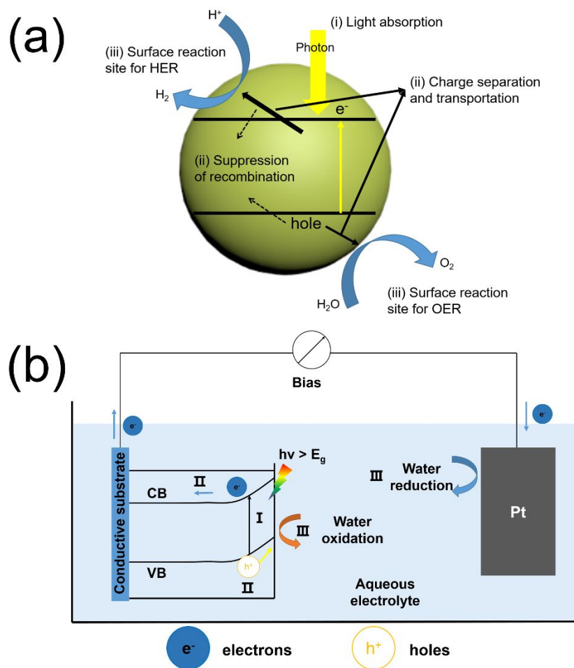
Fig. 1. (a) Schematic of the main process of PC water splitting in a simple photocatalytic semiconductors; (b) Diagram of a typical PEC water splitting system with an n-type semiconductor as the photoanode and Pt as the counter electrode, both immersing in aqueous electrolyte. In the picture, process I refers to photon absorption and the resulted excitation of an electron from VB to CB, leaving a hole at VB. Process II refers to the separation and transportation of photogenerated electron and hole pairs. Process III refers to the surface redox reactions, where water oxidation occurs at the semiconductor surface and the reduction reaction occurs at the Pt surface.
