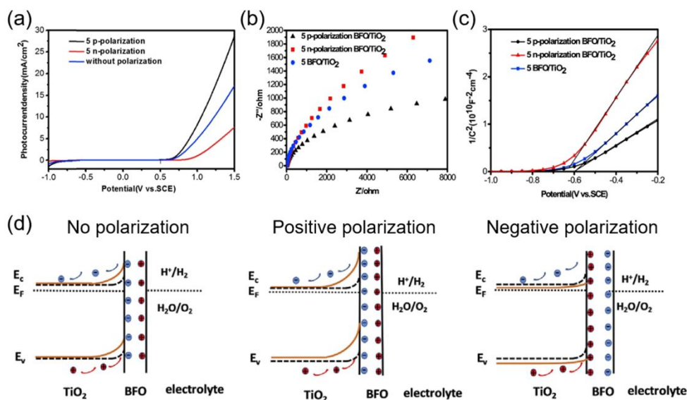
Fig. 8. BFO/ \text{TiO}_2 photoanode for PEC water splitting. (a) J_{\text{ph}}-V curves of positively, negatively poled and unpoled of \text{BFO}/\text{TiO}_2 under AM 1.5 G. (b) Nyquist plots and (c) Mott-Schottky plots of positively, negatively poled and unpoled \text{BFO}/\text{TiO}_2 under visible light. (d) Schematic band diagram of the \text{BFO}/\text{TiO}_2 photoanode interfacing with electrolyte without poling (left), and with positive (middle) and negative (right) poling, respectively. Reprinted from ref 104. Copyright 2019 Elsevier.
