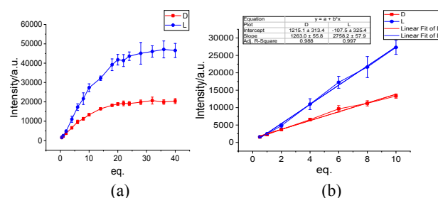
Figure 2. (a) Fluorescence intensity of ( S )- 2c @PEG-PLLA (10 μM) and Zn(OAc) 2 (2 equiv) at λ = 545 nm versus the stoichiometry of tryptophan. (b) Expanded view of 0.5 to 10 equiv tryptophan. (λ ex = 430 nm, slit = 3/3 nm, integration time = 0.1 s).
