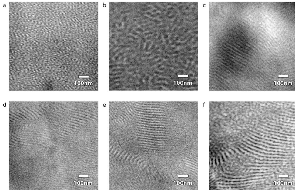
Figure 3. TEM images for microtomed and stained RIPT dog bone samples. a) \varphi_{\text{SBS}} = 100\% , b) \varphi_{\text{SBS}} = 50\% , c) \varphi_{\text{SBS}} = 40\% , d) \varphi_{\text{SBS}} = 30\% , e) \varphi_{\text{SBS}} = 20\% , and f) \varphi_{\text{SBS}} = 10\% . Samples were stained with \text{OsO}_4 .
