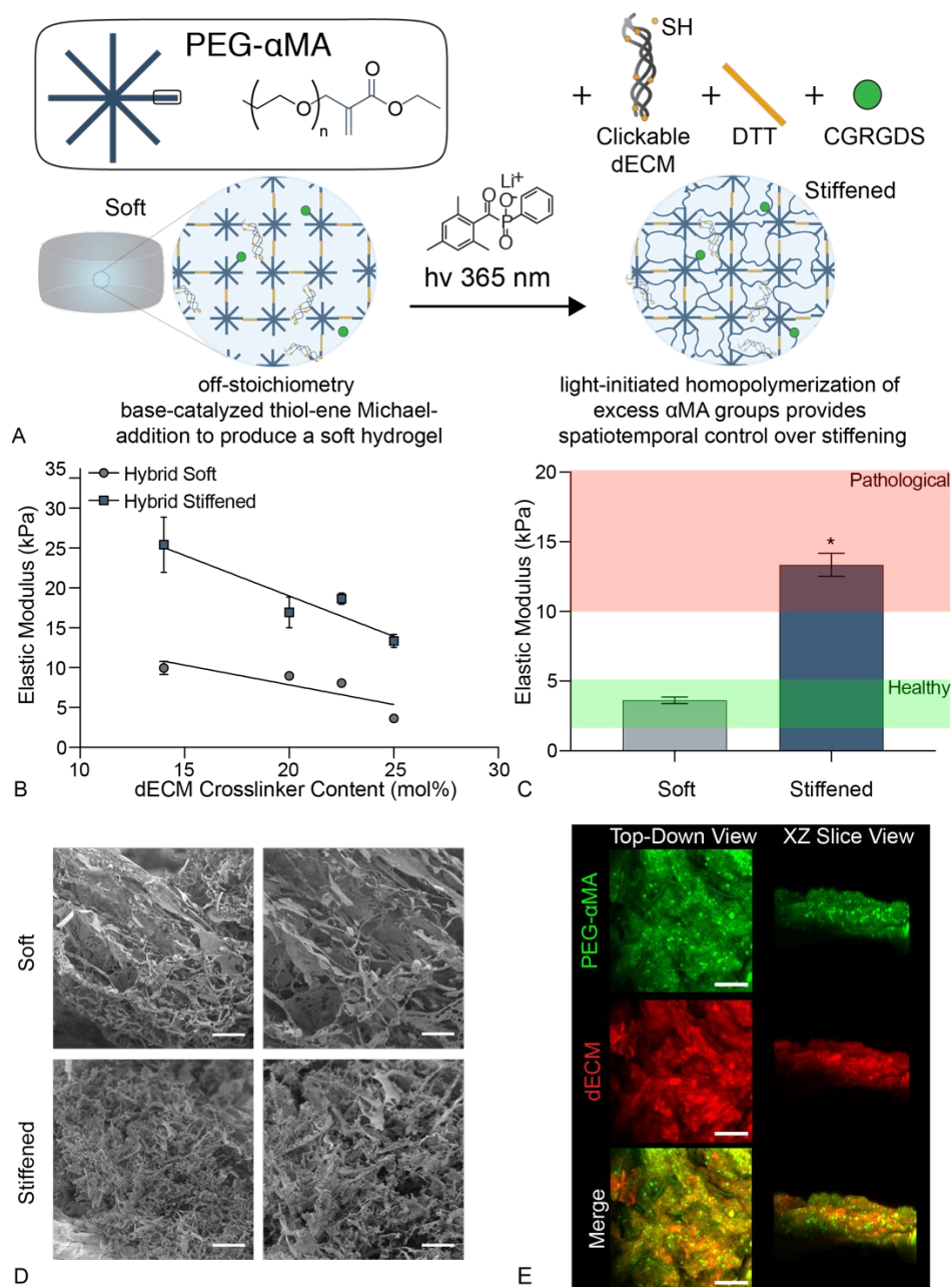
Fig. 2 A) Schematic of the dual-stage polymerization reaction that combined PEG \alpha MA and the clickable dECM crosslinker with DTT and CGRGDS to enable spatiotemporal control over stiffening. B) The elastic modulus of soft and stiffened hybrid hydrogels decreased with increasing dECM content ranging from 14 mol% to 25 mol% dECM ( n=4 , mean \pm SEM). C) Hybrid hydrogel formulations were adjusted so that soft and stiffened samples resulted in elastic modulus values within healthy and pathologic ranges, respectively ( n=4 , mean \pm SEM, *: p < 0.05 , ANOVA, Tukey test). D) Scanning electron micrographs of soft and stiffened hybrid hydrogels. Scale bars, 25 \mu m. E) Representative confocal images of hybrid hydrogels stained for PEG \alpha MA (green) and dECM (red) show uniform mixing of the two components throughout the samples. Scale bars, 50 \mu m.
