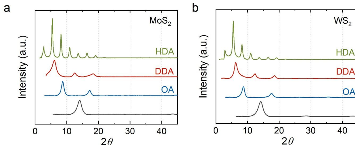
Figure 3. XRD of the n-alkylamine intercalated (a) MoS 2 and (b) WS 2 . Green: hexadecylamine-intercalated; red: dodecylamine-intercalated; blue: octylamine-intercalated; dark gray: restacked.
