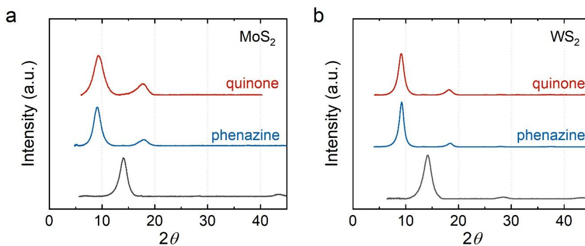
Figure 4. XRD of electro-proton transfer mediator intercalated (a) MoS 2 and (b) WS 2 . Red: p -benzoquinone-intercalated; blue: phenazine-intercalated; dark gray: restacked.
