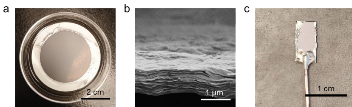
Figure 1. (a) Optical image of a representative restacked MoS 2 film on a nitrocellulose membrane. (b) SEM cross sectional image of a representative restacked MoS 2 film. (c) Optical image of an electrode prepared by transferring a restacked MoS 2 film onto a gold substrate. The edges of the electrode were sealed using silver paint.
