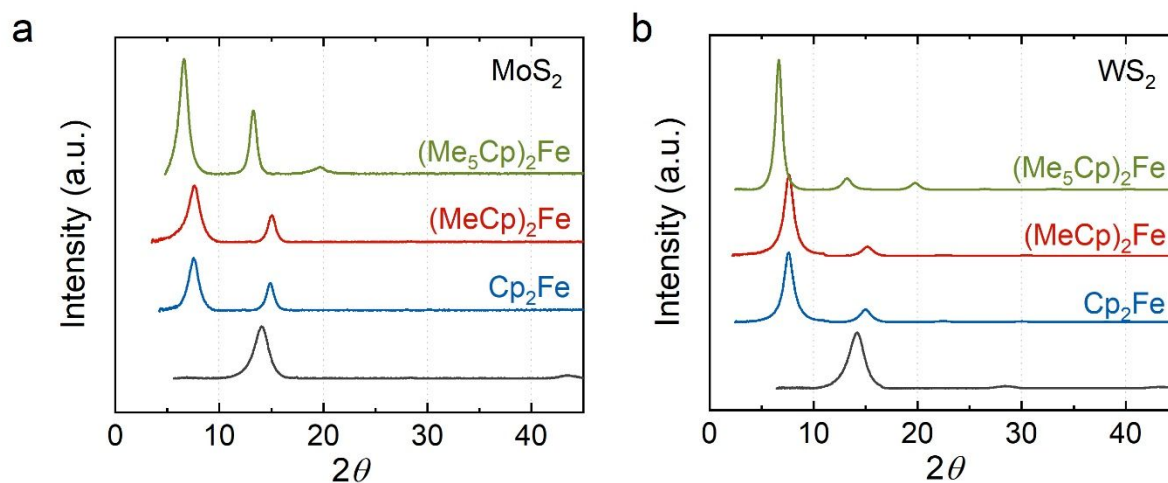
Figure 2. XRD of metallocene intercalated (a) \text{MoS}_2 and (b) \text{WS}_2 . Green: decamethylferrocene-intercalated; red: 1,1'-dimethylferrocene-intercalated; blue: ferrocene-intercalated; dark gray: restacked.
