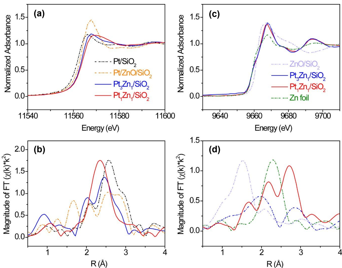
Figure 3. Pt L 3 edge (a) XANES and (b) EXAFS Fourier transform of Pt/SiO 2 , Pt/ZnO/SiO 2 , Pt 1 Zn 1 /SiO 2 , Pt 3 Zn 1 /SiO 2 . (c) Zn K edge XANES and (d) EXAFS Fourier transform of Zn, ZnO/SiO 2 , Pt 1 Zn 1 /SiO 2 , Pt 3 Zn 1 /SiO 2 .
