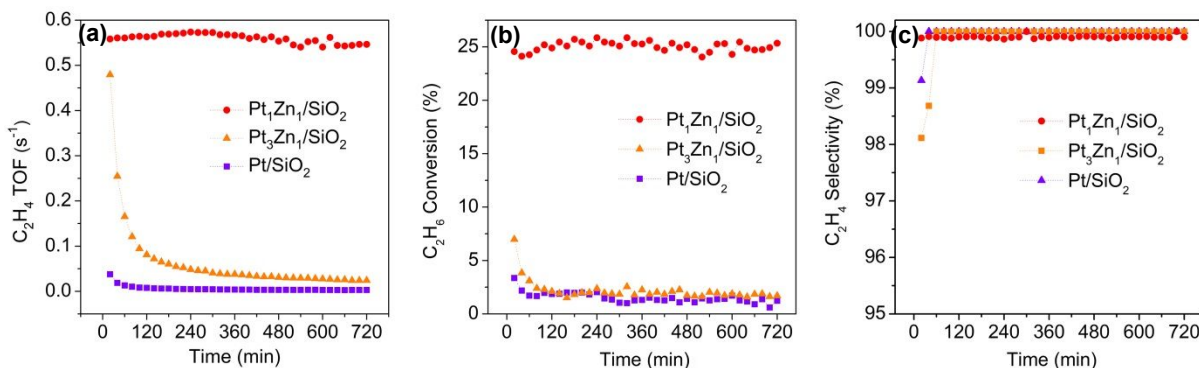
Figure 7 (a) \text{C}_2\text{H}_4 TOF \text{s}^{-1} , (b) \text{C}_2\text{H}_6 conversion and (c) \text{C}_2\text{H}_4 selectivity as a function of reaction time (reaction conditions: T = 550\text{ }^\circ\text{C} , \text{C}_2\text{H}_6 = 18\% with balance He. 100 mg catalyst was used for each test. All catalysts were pre-treated with 5% \text{H}_2/\text{He} for 30 min at 600\text{ }^\circ\text{C} before DHE, \text{WHSV} = 7.2\text{ h}^{-1} ).
