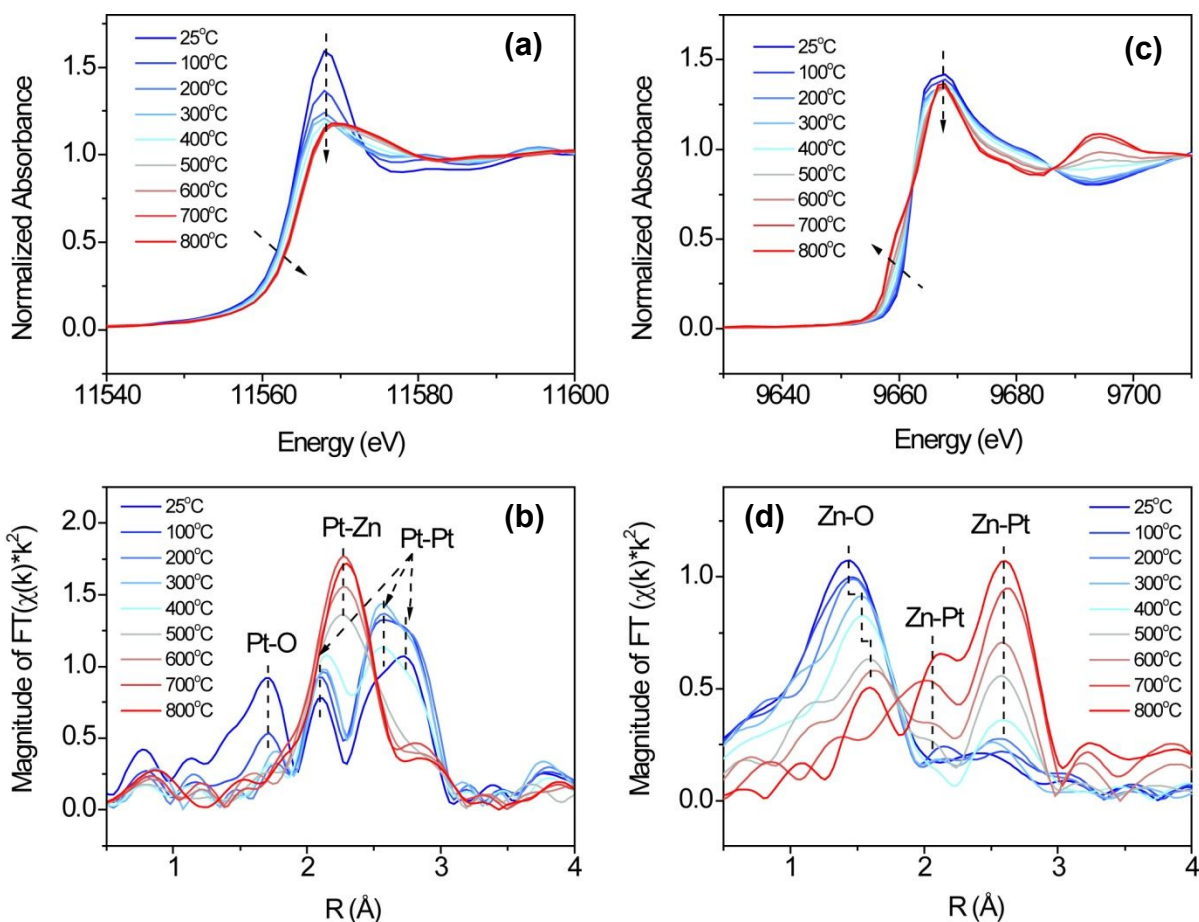
Figure 5. Pt L 3 edge (a) XANES, (b) EXAFS Fourier transform of Pt/ZnO/SiO 2 during in situ hydrogen reduction at elevating temperatures and their Zn K edge XANES (c) and (d) EXAFS counterparts.
