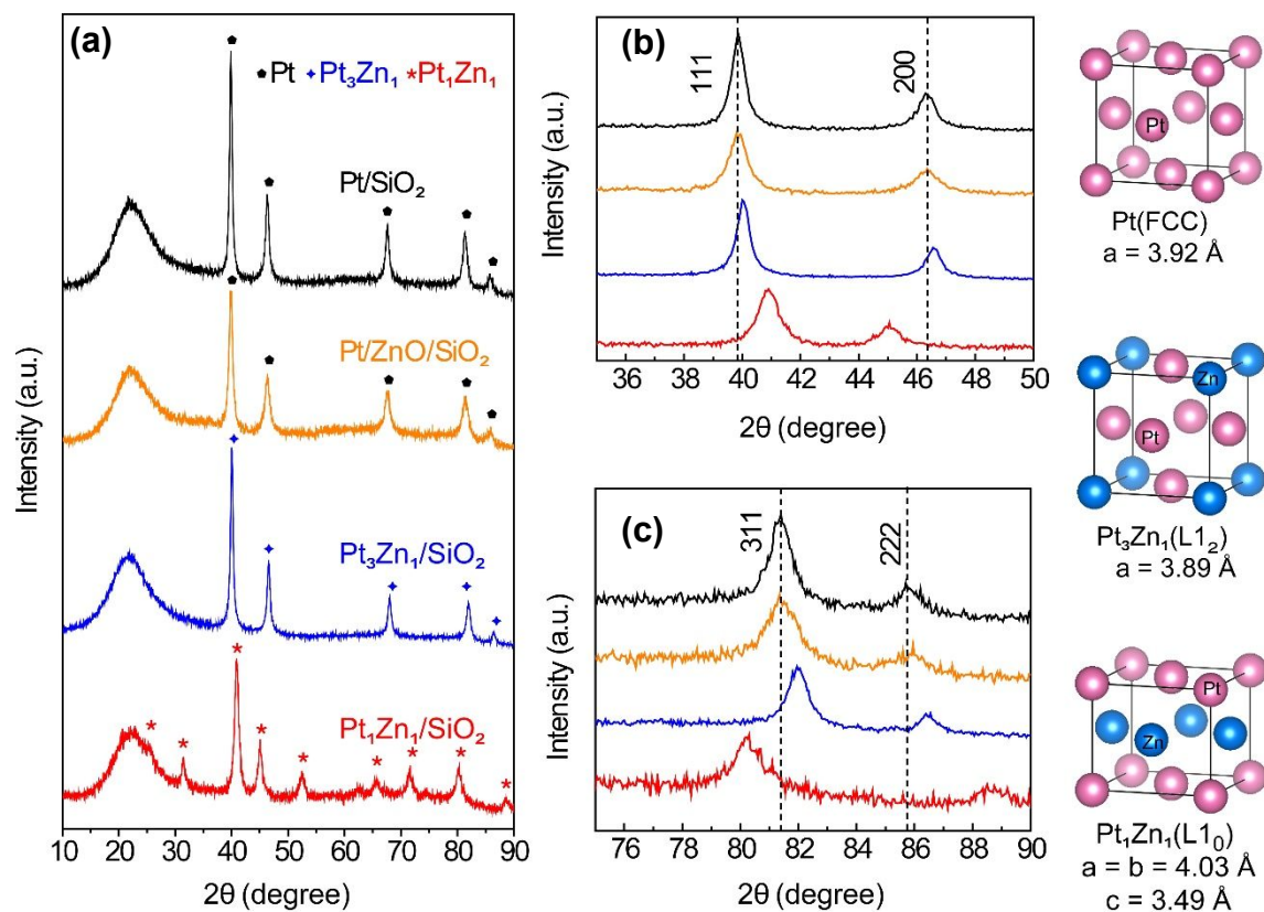
Figure 2 (a) XRD patterns of Pt/SiO 2 , pre-catalyst Pt/ZnO/SiO 2 , Pt 3 Zn 1 /SiO 2 and Pt 1 Zn 1 /SiO 2 . Detailed scans of XRD patterns of the four samples between (b) 35°-50° and (c) 75°-90°.
