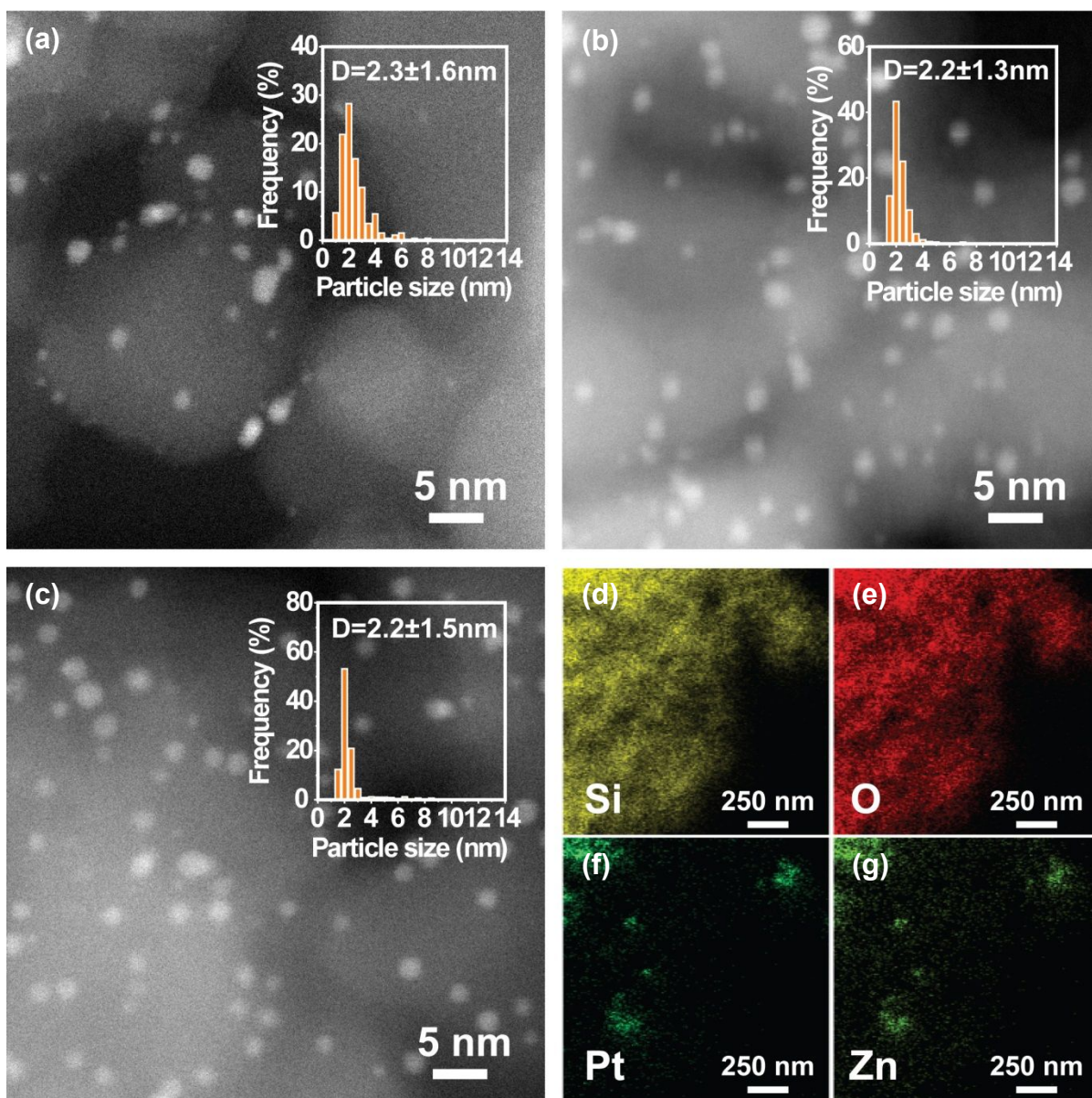
Figure 4. (a-b) HAADF-STEM images and particle size distribution histograms of (a) Pt/SiO 2 , (b) Pt 3 Zn 1 /SiO 2 , (c) Pt 1 Zn 1 /SiO 2 , and (d-g) EDX mapping of Pt 1 Zn 1 /SiO 2 .
