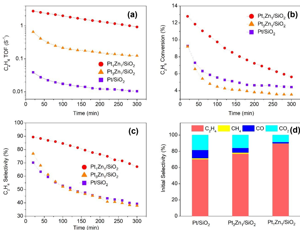
Figure 8. (a) C 2 H 4 TOF, (b) C 2 H 6 conversion and (c) C 2 H 4 selectivity as a function of reaction time. (d) Initial selectivity of the product gases on the catalysts. (Reaction conditions: T = 550 °C, C 2 H 6 = 22.3%, O 2 = 1.7%, He = 76%, total flowrate = 50 ml/min. All catalysts were pre-treated with 5% H 2 /He for 30 min at 600 °C before ODHE, initial conversion was at ~10% for all catalysts).
