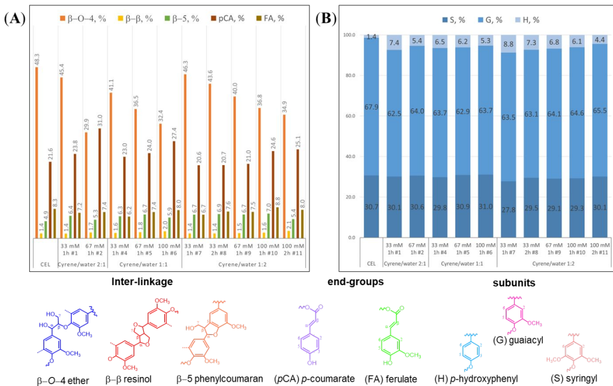
Figure 4. Semi-quantitative HSQC analysis of switchgrass CEL and Cyrene lignin. Frequencies of lignin inter-unit linkages ( \beta\text{-O-4} ether, \beta\text{-}\beta resinol and \beta\text{-}5 phenylcoumaran) and end-groups ( p -coumarate and ferulate) (A), and subunits (guaiacyl, syringyl, p -hydroxyphenyl) (B) per 100 (S+G+H) units.
