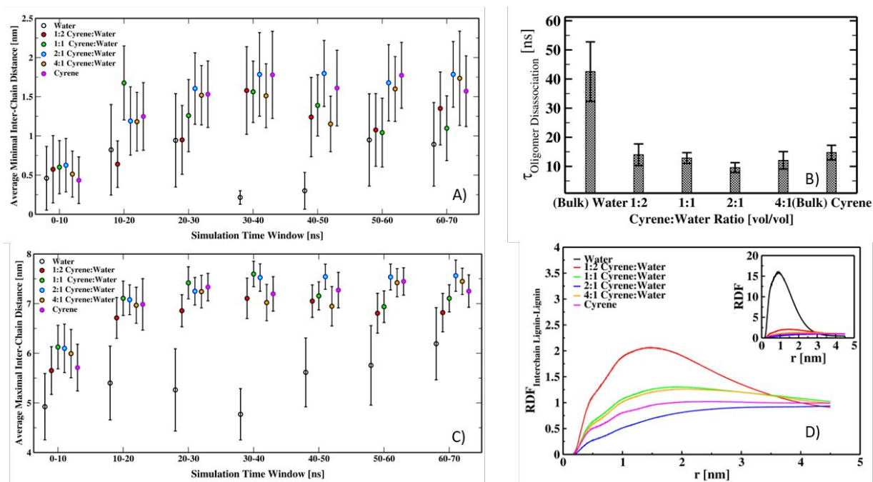
Figure 5. Lignin aggregate characterization. (A) Average minimal distances between inter-lignin chains obtained over 10ns windows from 5 independent simulations. (B) Bar-graph representation of mean first exit times for the disassociation of a lignin chain from other lignins. A disassociation event is taken as the time when the minimal distance to any other lignin chains is more than 1.5nm. (C) Average maximal distances between inter-lignin chains obtained over 10ns windows from 5 independent simulations. (D) Inter-chain, monomer-centered, lignin-lignin radial distribution functions; radial distribution functions were calculated using the last 25ns of each of the five-independent 70ns trajectories per solvent condition. Error-bars presented in subfigures are standard deviations.
