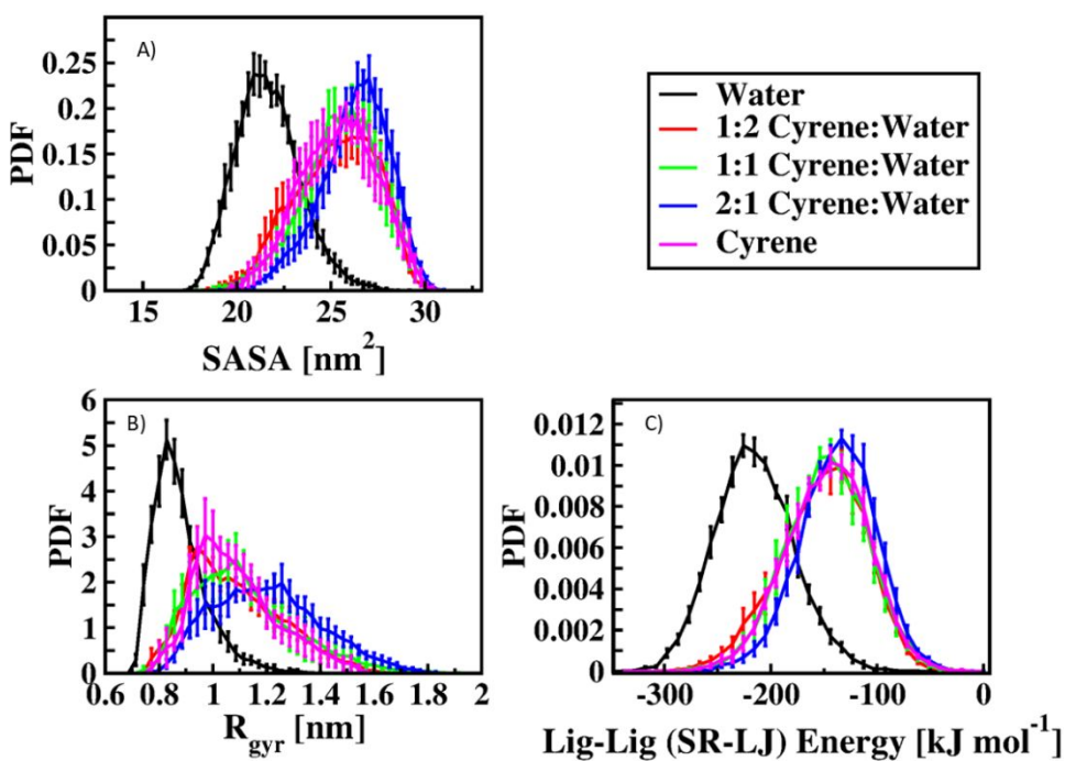
Figure 6. Isolated lignin chain characteristics under water, Cyrene, and cosolvent conditions. (A) Mean lignin solvent accessible surface area distributions. (B) Mean lignin radius of gyration distributions. (C) Mean short-range intra-chain (lignin-lignin) Lennard-Jones interaction energy distributions. All distributions were obtained by histogramming calculated features over the final 10ns of each (five) independent trajectory for each of the solvent conditions. Error-estimates are standard-errors for each bin assignment. Lennard-Jones energies are used to approximate the strength and number of close intra-chain contacts. This is necessarily an incomplete measure of contact energies as it excludes electrostatic contributions though it does provide a window into potential contact screening.
