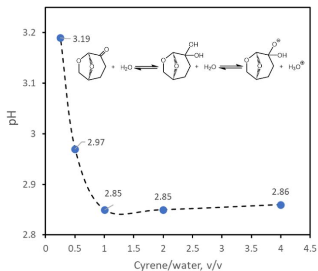
Figure 1. The correlation between pH and Cyrene/water ratio.
