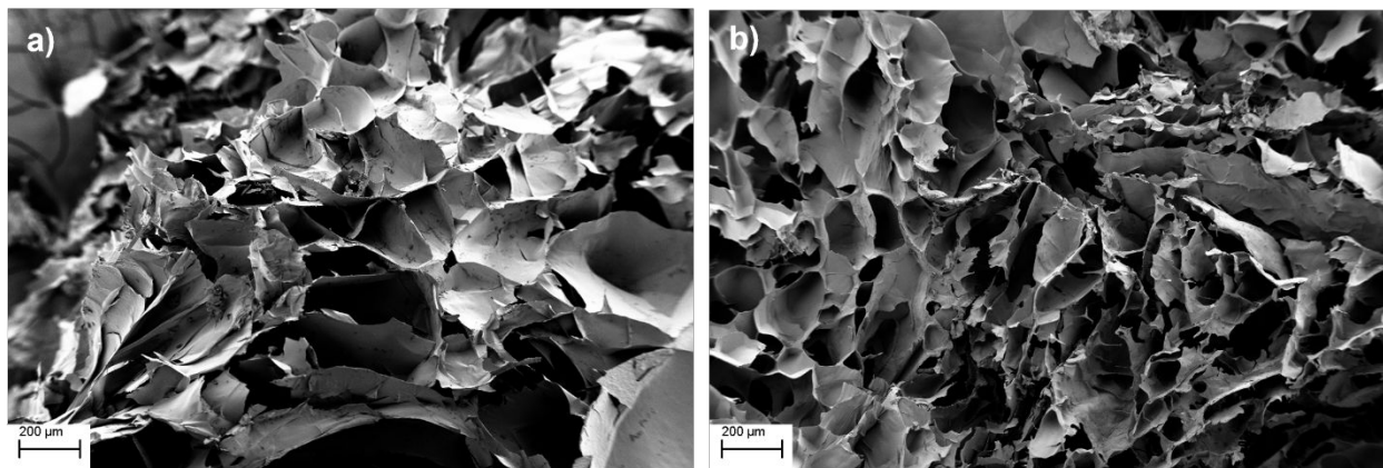
Figure 1: SEM images of a) 2 wt% and b) 4 wt% chitosan scaffolds. 50x magnification, scale bars 200 \mu\text{m} .
