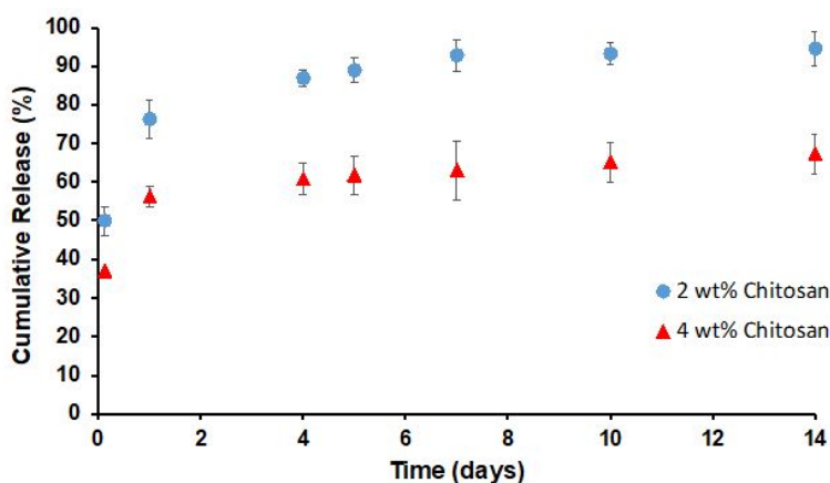
Figure 5: \alpha -chymotrypsin release from 2 and 4 wt% chitosan scaffolds in 1x PBS at 37°C, pH 7.4. Data shown are mean \pm SD (n=3).
