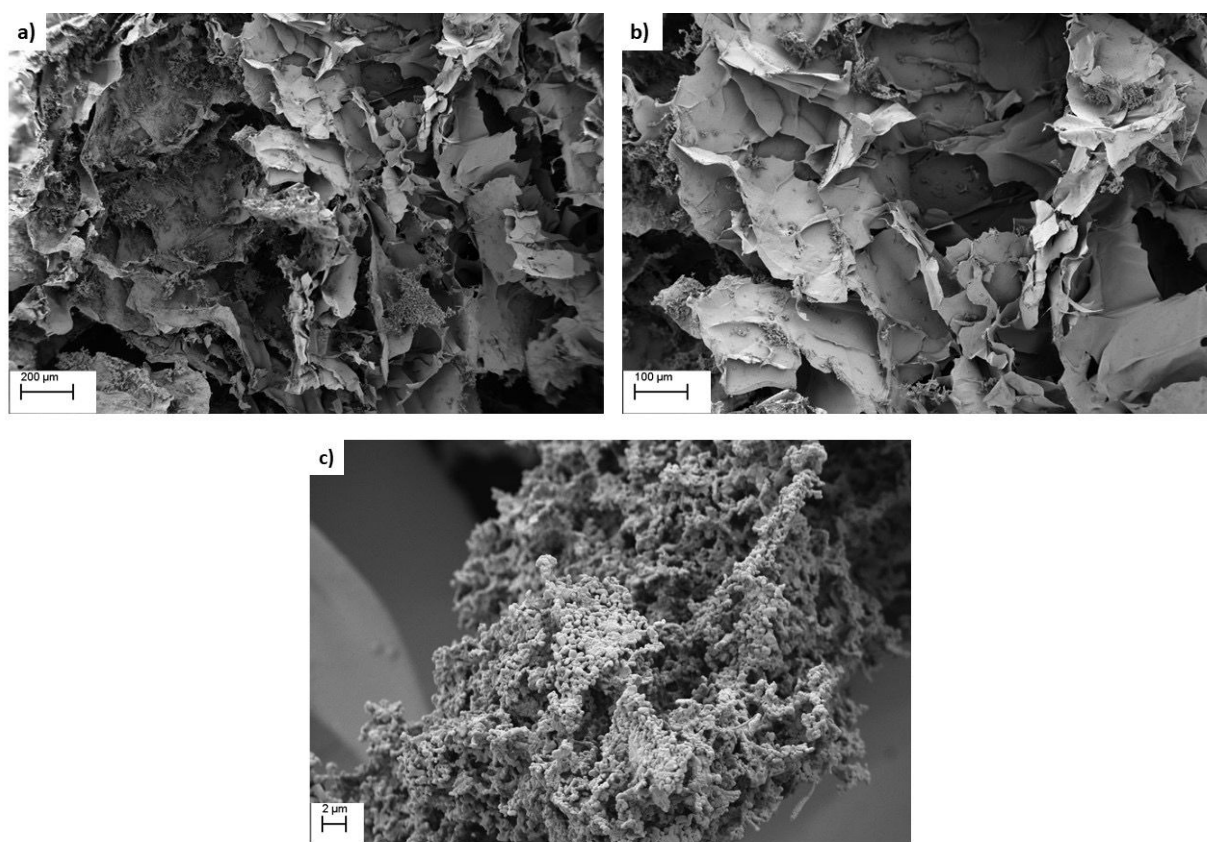
Figure 6: SEM images of scaffolds with conjugated P(MMA-co-MAA) nanoparticles taken at a) 50x b) 100x and c) 2240x magnification.
