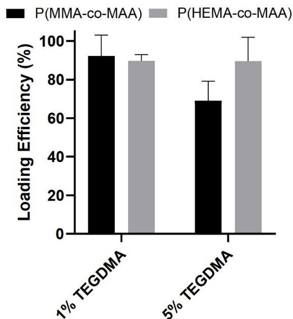
Figure 3: Loading efficiencies of FITC- \alpha -chymotrypsin loaded into P(MMA-co-MAA) and P(HEMA-co-MAA) nanoparticles crosslinked with 1 and 5 mol% TEGDMA. Loading was performed in 0.1x PBS at 25°C, pH 7.4. Data shown are mean \pm SD (n=3).
