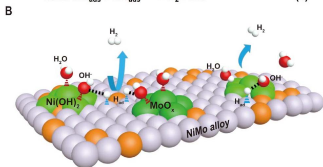
Fig. 1 (A) The reaction mechanism for the HER in alkaline electrolytes and two pathways are presented in the forms of the Volmer–Heyrovsky mechanism and the Volmer–Tafel mechanism. (B) Schematic diagram of synergistic catalysis of alloy–oxide or alloy–hydroxide interface structures, in which the oxide or hydroxide promotes water dissociation and the alloy accelerates hydrogen combination.
