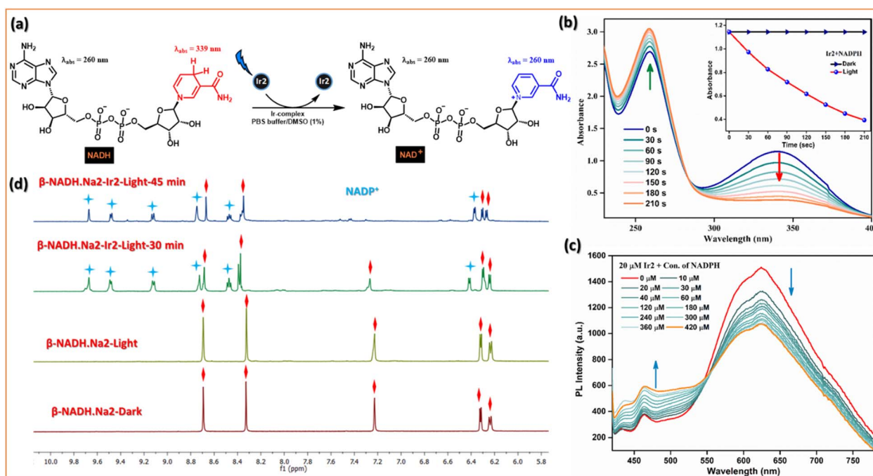
Fig. 6 Photocatalytic oxidation of NADH. (a) Schematic illustration of photocatalytic NADH/ NAD^+ transformation by Ir2 under light irradiation. (b) Reaction of Ir2 (10 \mu M ) and NADH (200 \mu M ) in PBS solution under blue LED light irradiation monitored by UV-vis absorption spectra at 298 K. The inserted picture shows TON of Ir2 under dark or irradiation conditions. (c) Stern–Volmer quenching for the interaction of different conc. of NADH with the excited state of Ir2. (d) Photooxidation of NADH (3.5 mM) by Ir2 (0.25 mM) under dark or irradiation conditions monitored by ^1H NMR spectroscopy at 298 K. Peaks associated with blue stars represent NAD^+ , and those with red squares represent NADH.
