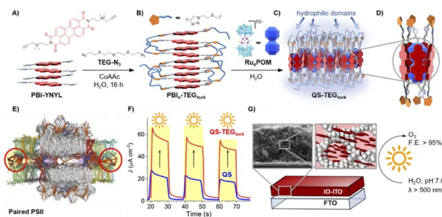
Fig. 18 Second-generation quasosomes, exploiting an inter-locked multi-chromophoric antenna system based on PBI photosensitizers bearing hydrophilic tetraethylene glycol chains (TEG). Reprinted from ref. 39 with permission from the American Chemical Society, copyright 2022.
