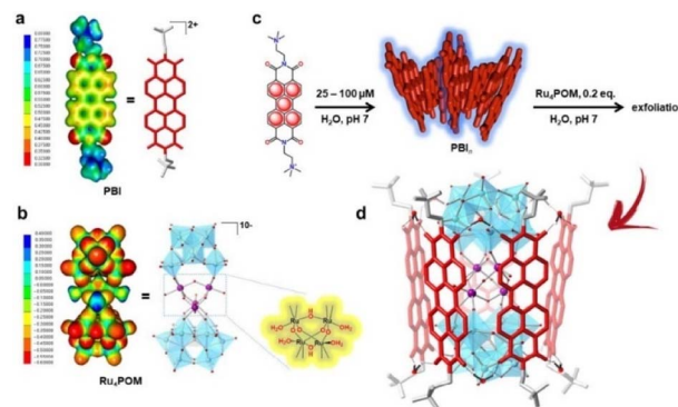
Fig. 17 Self-assembly in water of artificial quasosomes (QS) from a dicationic perylene bisimide \text{PBI}^{2+} and a decaanionic \text{Ru}_4\text{POM} WOC. Reprinted from ref. 117 with permission from the Nature Publishing Group, copyright 2019.
