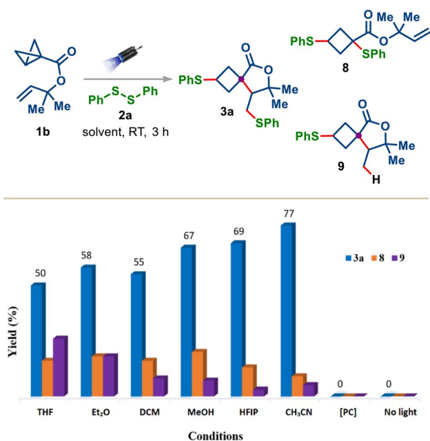
Fig. 1 Optimization of the reaction conditions. Reactions were carried out under an inert atmosphere. Conditions: 1b (0.15 mmol), 2a (0.15 mmol), solvent (1.5 mL, 0.1 M), 457 nm photocube, 3 h. [PC] = [\text{Ir}(\text{d}(\text{CF}_3)\text{ppy})_2(\text{dtbbpy})]\text{PF}_6 . Yields were determined by ^1\text{H} -NMR using \text{CH}_2\text{Br}_2 as the internal standard. Depending on the solvent, dr varied between 1.7 : 1 to 1.2 : 1 (see the ESI†).
