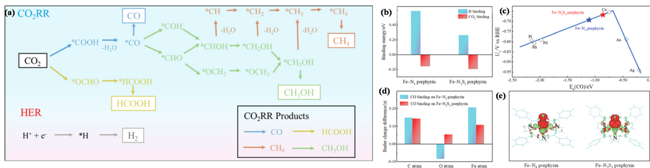
Fig. 25 (a) The schematic of elementary steps of the \text{CO}_2\text{RR} . (b) \text{CO}_2 and H binding energies. (c) Volcano plot. (d) Bader charge difference of C and O atoms of the CO molecule and Fe atom before and after CO binding. (e) Charge density difference of CO binding. Reproduced with permission. 203 Copyright 2021, Wiley-VCH GmbH.
