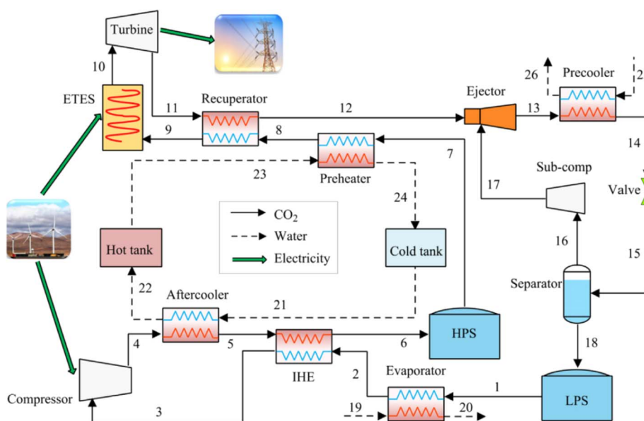
Fig. 2 A schematic of the carbon dioxide electrothermal energy storage system's cycle. 43
