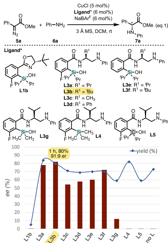
Fig. 2 Ligand optimization for enantioselective N–H insertion of α-phenyl-α-diazoester with aniline (see ESI† for raw data). Standard reaction conditions: 5a and 6a (0.2 mmol, 1.0 equiv. each) in DCM (0.05 M) at 23 °C in 1 h; L3c in 2 h. L1b required 16 h for 74% (60 : 40 er, opposite enantiomer); however, 1 h timepoint for L1b is graphed for direct comparison. Yield determined using NMR spectroscopy with Ph-TMS as internal standard. Enantiomeric excess (ee%) determined using CSP-HPLC analysis with a Chiralpak OD-H column.
