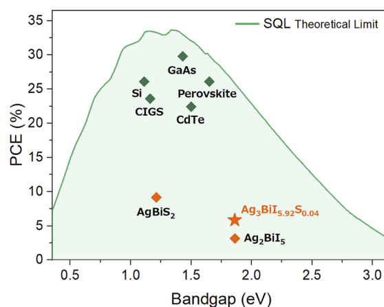
Fig. 1 Power conversion efficiency vs. band gap energy, illustrating the highest efficiencies for various solar cells.
