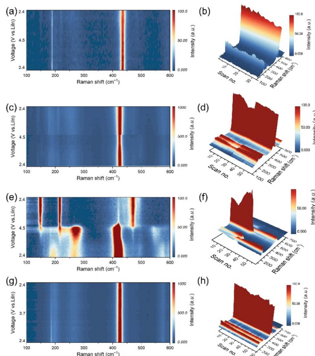
Fig. 2 The in situ Raman spectra of (a and b) LPSCl-VGCF|LPSCl|LiIn, (c and d) uncoated LNMO-LPSCl-VGCF|LPSCl|LiIn, (e and f) LTA@LNMO-LPSCl-VGCF|LPSCl|LiIn, and (g and h) LCO-LPSCl-VGCF|LPSCl|LiIn cells from two-dimensional and three-dimensional views, respectively. The positions for Raman signal collection are the LPSCl-rich area far from the cathode active particle/LPSCl particle interface in the composite cathode.
