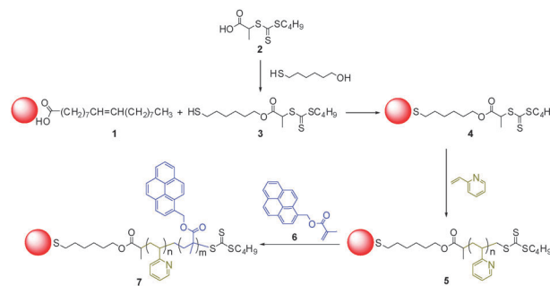
Scheme 1 Synthesis of (PyMMP- b -P2VP)-CdSe/ZnS QDs.
