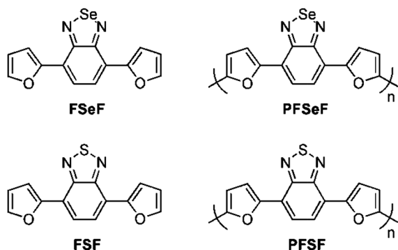
Scheme 1 Chemical structures of FSeF , FSF monomers and their corresponding polymers PFSeF and PFSeF .
