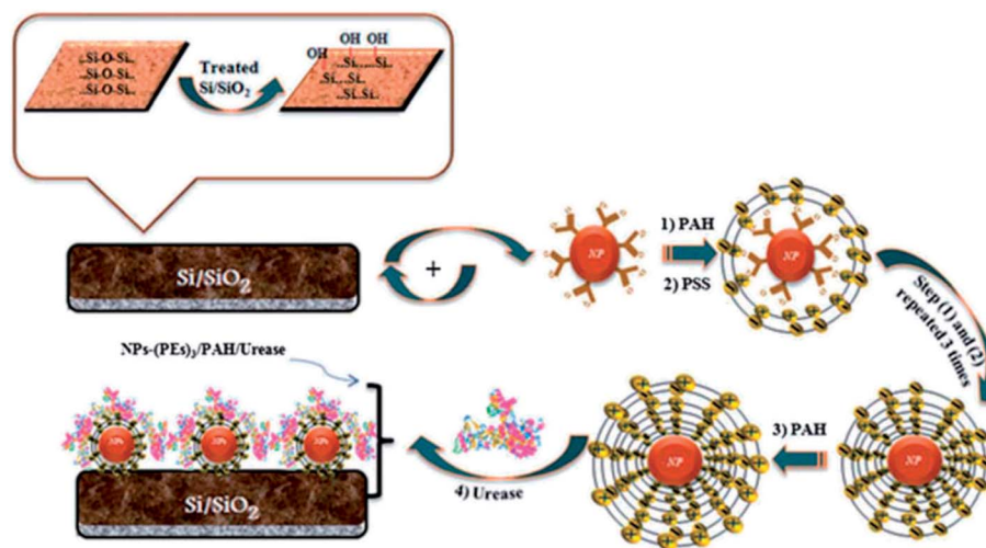
Fig. 12 Biosensor construction using Fe 3 O 4 and polyelectrolyte materials for atrazine detection. Reproduced with permission from ref. 187 © 2013 Royal Society of Chemistry.
