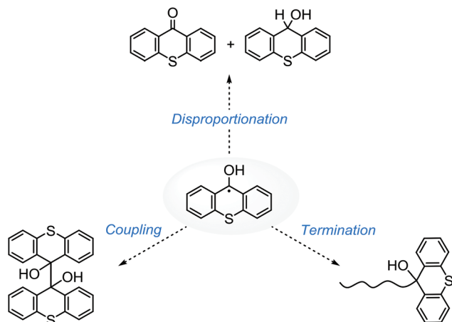
Scheme 4 Possible reactions of thioxanthy ketyl radicals.
