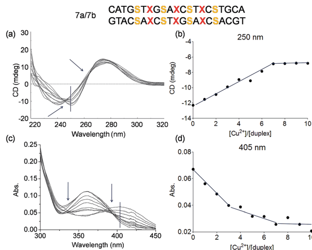
Fig. 8 Schematic depiction of the investigated duplex, S = salen, X = pyrazole. (a) Overlaid CD spectrum at different concentrations of Cu 2+ (from 0 to 10 eq.) of the duplex 7a/7b ; (b) plot of circular dichroic changes at 250 nm against the ration of [Cu 2+ ]/[ 7a/7b ]; (c) overlaid UV spectrum under the same conditions as in (a); (d) plot of UV absorbance at 405 nm against the ration of [Cu 2+ ]/[ 7a/7b ]. Conditions: 150 mM NaCl, 10 mM CHES buffer pH 9.0, 3 μM oligonucleotide, 30 eq. ethylenediamine, final volume of 200 μL.
