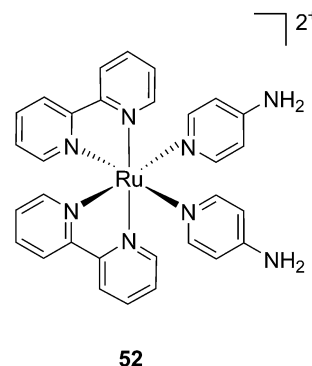
Fig. 36 Structure of the \text{Ru}(\text{II}) caged neuroactive 4-AP. 104
