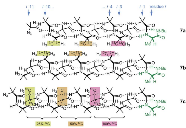
Fig. 6 Multi-labelled oligomers 7a–c allow measurement of screw sense at each of the nine positions in the oligomer from i-3 to i-11 .
