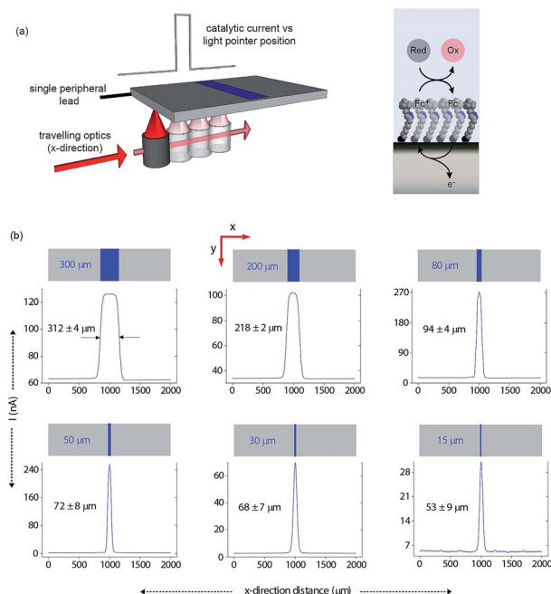
Fig. 3 Direct measurements of the size of a 2D surface redox feature through a single peripheral connection. (a) A schematic of the experimental design where a travelling, collimated focused light beam ( \sim 80 \mu\text{m} FWHM, \lambda = 642 nm, optical power is 0.1 mW, Fig. S4 in ESI†) moves along the x-direction to illuminate the backside of a macroscopic n-type silicon electrode. On the upper side is exposed to 1 mM [\text{Fe}(\text{CN})_6]^{4-}/100 mM \text{KNO}_3 electrolyte solution and contains a patterned ferrocene feature (blue area) of known width. The faradaic current is recorded as a function of the light pointer position. (b) Current measurements for electroactive features on a monolithic electrode of 300 \mu\text{m} , 200 \mu\text{m} , 80 \mu\text{m} , 50 \mu\text{m} , 30 \mu\text{m} and 15 \mu\text{m} width. The minimal lateral spacing of adjacent features that can be resolved is close to the substrate thickness. Note that the adsorption depth for red radiation in silicon is < 4 \mu\text{m} , and the substrate thickness is 55 \pm 6 \mu\text{m} .
