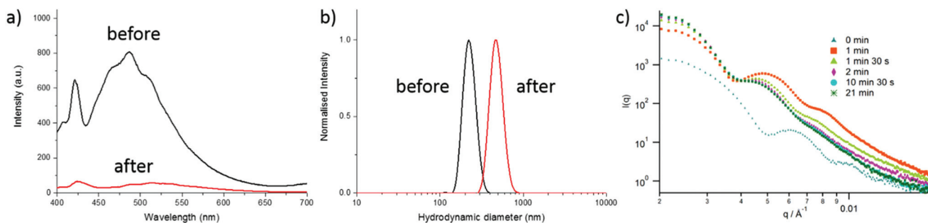
Fig. 2 (a) Fluorescence emission spectra of particles 8 before and after the first CO 2 bubbling, (b) DLS of particles 8 before and after the first CO 2 purge, (c) in situ size monitoring of particles 3 by SAXS over 21 min of CO 2 bubbling.
