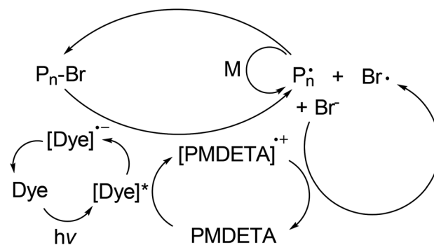
Scheme 1 Proposed mechanism of photoinduced, metal-free ATRP using dye/amine initiating system.
