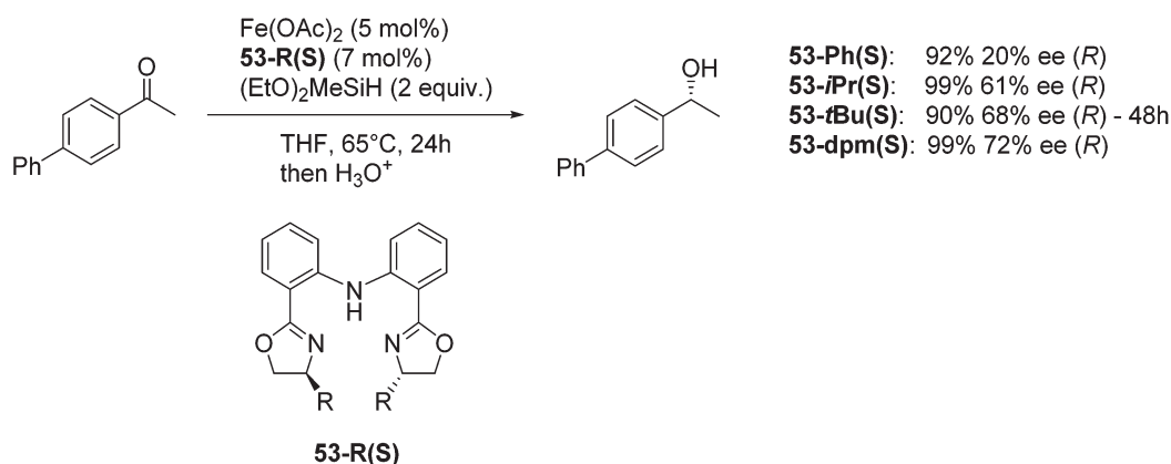
Fig. 21 Enantioselective hydrosilylation using the in situ formed iron catalyst.
