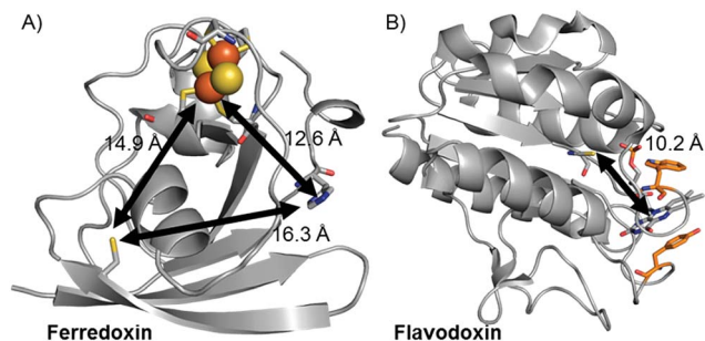
Fig. 2 Crystal structures of (A) Fd (1A70) 25 and (B) Fld (1CZL) 42 proteins with distances between possible binding sites for catalysts, PSs, and native redox cofactors. The closest relative distances between catalyst and PS binding sites and redox cofactors are indicated on the figure.
