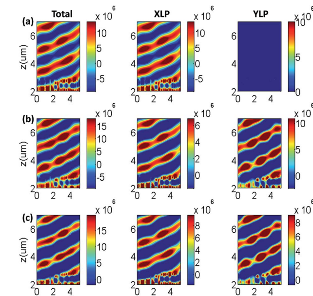
Fig. 4 Transmitted total, XLP and YLP electric field distributions of the metasurface illuminated with normal incidences of XLP light (a), 30° LP light (b) and 45° LP light (c) with the refractive angles of 17°.
