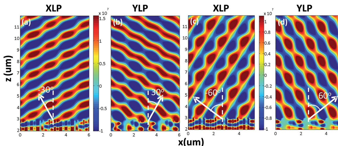
Fig. 3 Transmitted XLP (a and c) and YLP (b and d) electric field distributions of the metasurface illuminated with a normal incidences of 45° LP lights with the refractive angles of 30° (a and b) and 60° (c and d).
