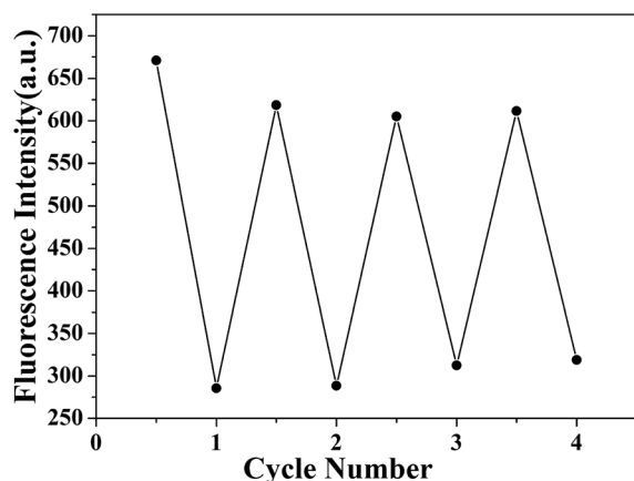
Fig. 4 Recycle use of PP5 for selective detection and facile removal of the toxic Hg^{2+} . Upon treatment in aqueous Na_2S solution, PP5 was easily recovered and could be repeatedly used.
