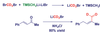
Scheme 14 Labelled experiments supporting the mechanism.
