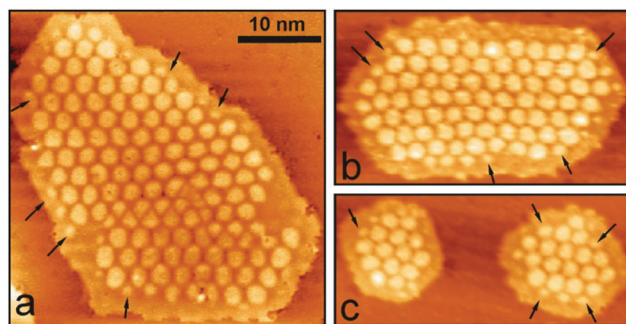
Fig. 26 STM images of the \text{FeO}_{2-x} islands after exposure to 10^{-6} mbar CO at 400 K for 4 min. Tunneling conditions: bias -3 V, current 0.05 nA. The arrows highlight non-uniform disappearance of the Moiré spots close to the island edge. 272 Reproduced with permission from ref. 272. Copyright 2015 Wiley-VCH.
