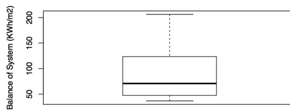
Fig. 1 Distribution in the cumulative electrical energy demand for the balance of system (CE e D BOS ) on a per unit area basis [kW h e m -2 ] from our meta-analysis. The 0, 25, 50, 75, and 100 percentile values are, respectively, 36.58, 47.52, 70.59, 123.55, and 206.36 kW h e m -2 .
