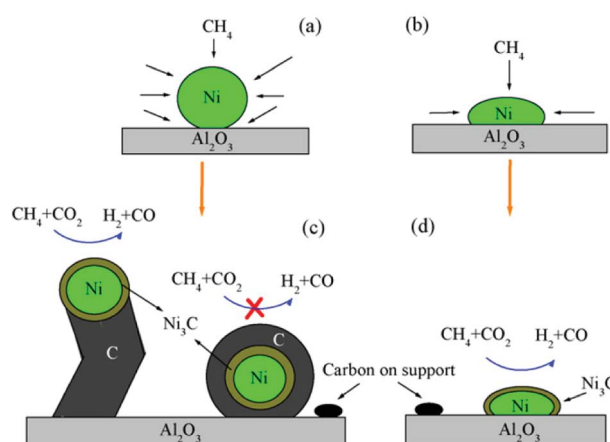
Fig. 3 Schematic representation of CO 2 /CH 4 reforming over (a and c) NiAl-C (calcinated); and (b and d) NiAl-PC (plasma treated prior to calcination) samples. Reproduced from ref. 161 with permission from Elsevier, copyright 2008.
