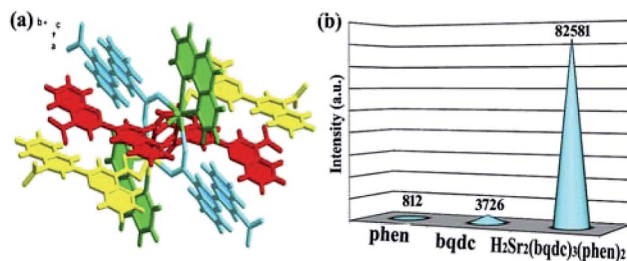
Fig. 2 (a) The crystal structure of the title complex. (b) The emission intensities of phen, bqdc and \text{H}_2\text{Sr}_2(\text{bqdc})_3(\text{phen})_2 .
