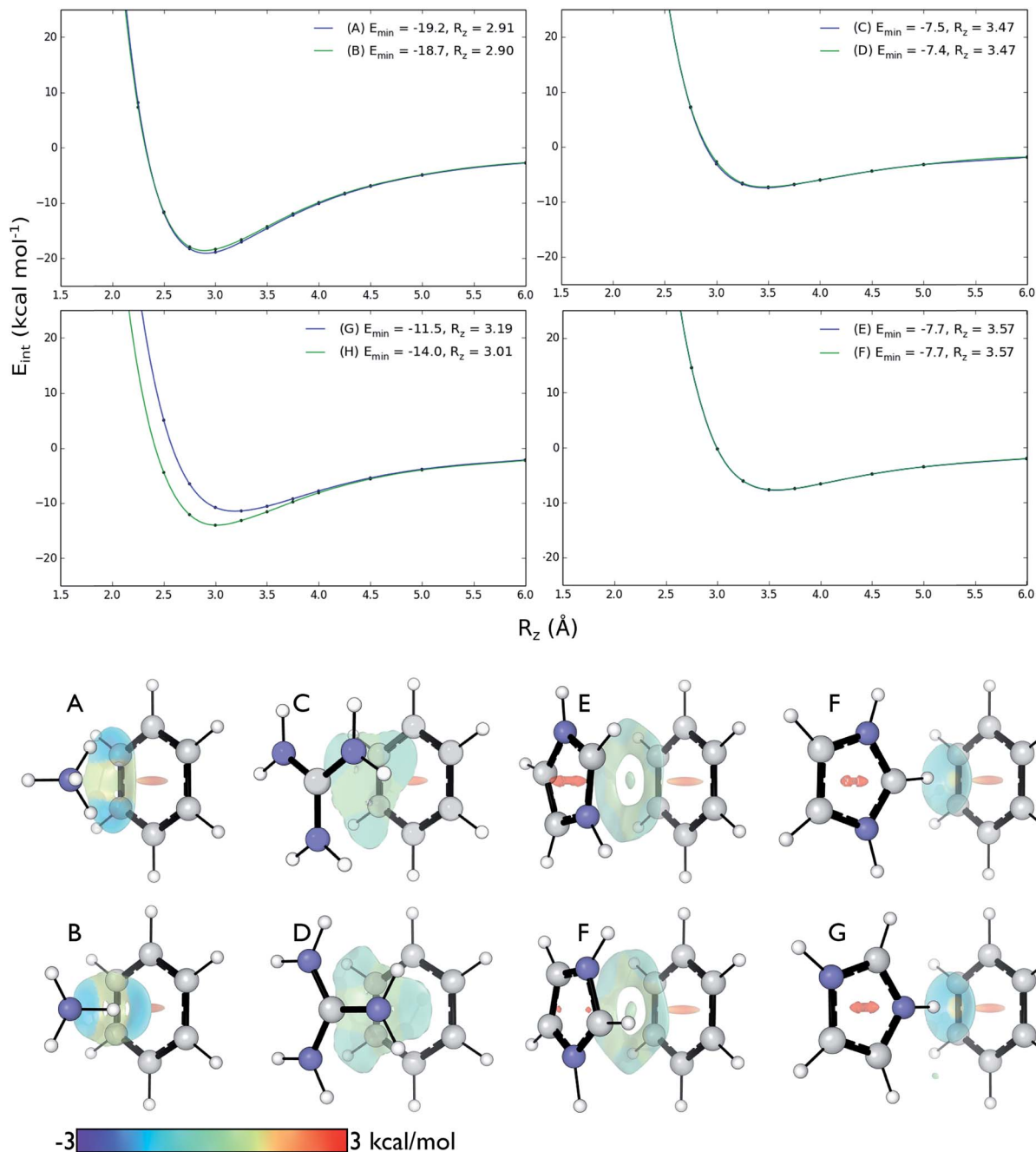
Fig. 4 Top: DLPNO-CCSD(T)/aug-cc-pVTZ interaction energies (kcal mol -1 ) as a function of intermolecular separation of cation-π complexes. Minimum energies ( E_{\text{min}} ) and equilibrium separations ( R_z ) shown. Bottom: NCI isosurfaces at the minimum energy separations.
