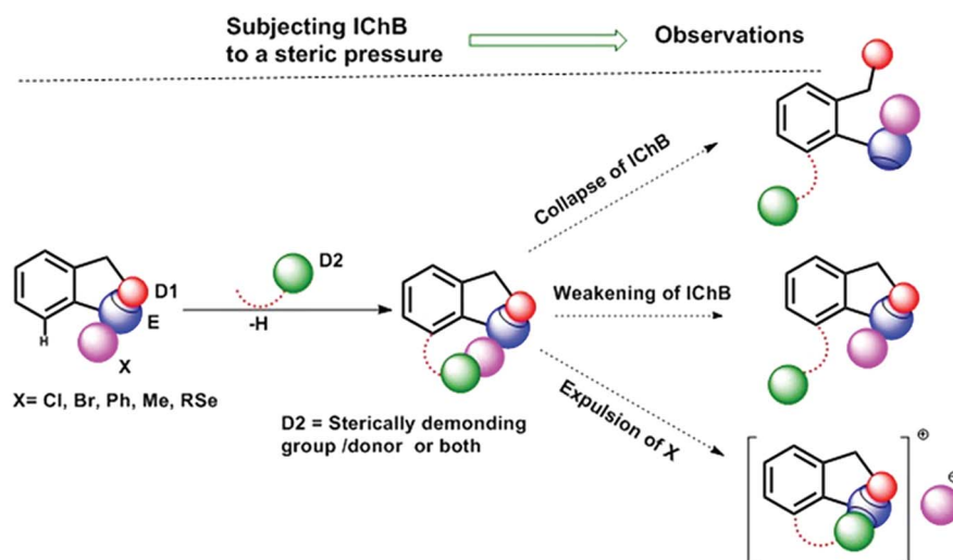
Fig. 2 The possible outcomes of subjecting IChBs ( D1 \cdots Se-X ) to additional steric stress. Replacement of the hydrogen atom present at the 6-position of the aryl ring with a sterically demanding group/donor or both leads to distinct structural and reactivity patterns.
