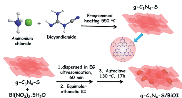
Fig. 1 Synthetic strategy of g-C 3 N 4 -S/BiOI heterojunction composite.
