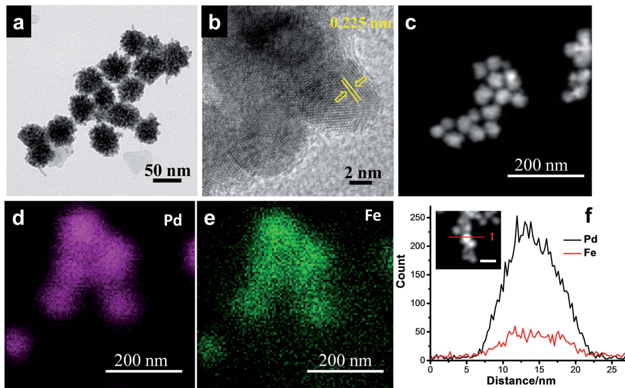
Fig. 3 (a) TEM, (b) HRTEM, and (c) HAADF-STEM images, and (d and e) elemental mapping and (f) EDS line scanning profiles of the \text{Pd}_{91}\text{Fe}_9/\text{GCN} nanohybrids.
