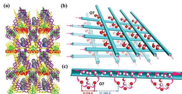
Fig. 12 Ionic transport pathway of FJU-66 [ EVIm ] OH . (a) Packing view of FJU-66 [ EVIm ] OH along the a direction. (b) Packing view of the available water pathways in FJU-66 along the a and b directions. (c) Possible supramolecular chain formed by \text{OH}^- anions and water molecules inside the channel of FJU-66 for efficient \text{OH}^- ion conduction. Reproduced from ref. 56 with permission from American Chemical Society, Copyright 2017.
