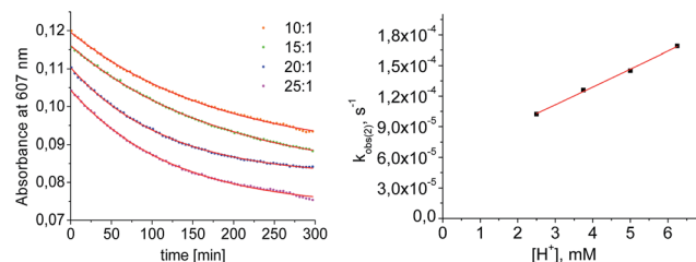
Fig. 4 Left: plot of the absorbance at 607 nm vs. time for different concentrations of [\text{HNEt}_3^+] . Results from fitting to the rate law are indicated by red lines. Right: plot of k_{\text{obs}(2)} vs. [\text{HNEt}_3^+] .
