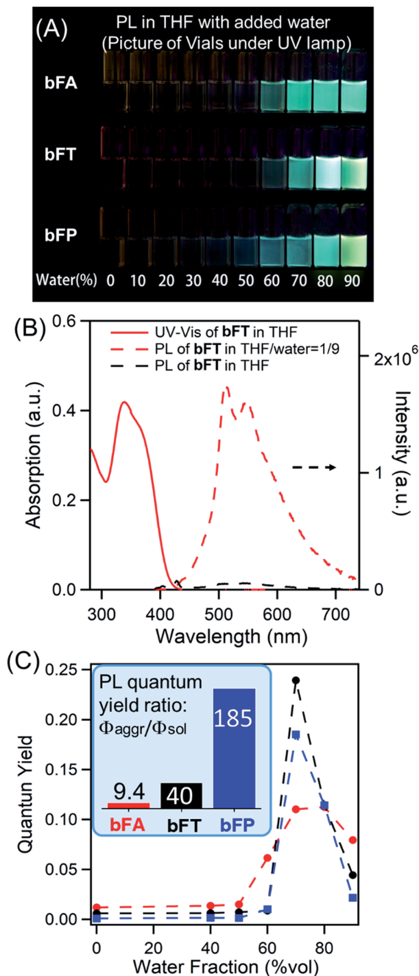
Fig. 2 (A) Photographic image of quartz vials containing difluoroenylidene acenequinoids displaying fluorescence in THF/H 2 O solutions with different water fractions irradiated using a 365 nm UV lamp; (B) UV-Vis and photoluminescence spectra of bFT in THF and THF/water = 1/9; (C) plots of quantum yield as a function of water fraction with excitation at 380 nm; the inset is the aggregation induced emission efficiency ( \Phi_{\text{aggr}}/\Phi_{\text{sol}} ); absolute quantum yields of these samples were determined with an integrating sphere (Horiba Fluorolog-3).
