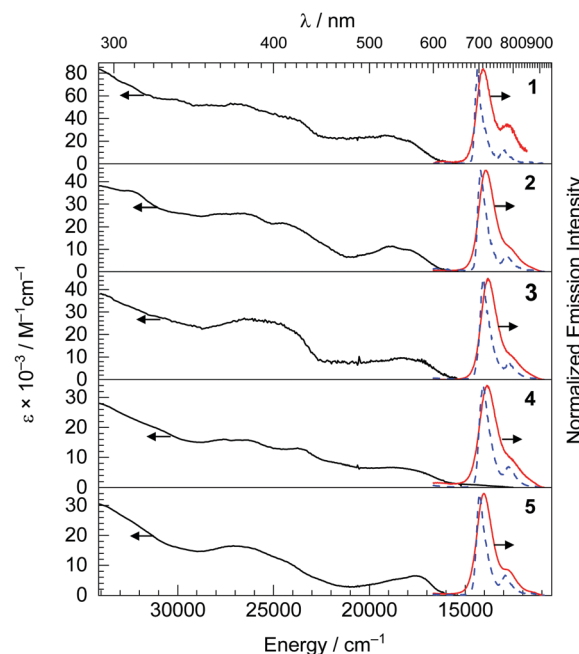
Fig. 2 Stacked plots of UV-vis absorption and room temperature PL emission spectra were measured in deaerated THF (black and red solid lines), along with 77 K PL emission spectra measured in toluene glass (blue dashed lines).
