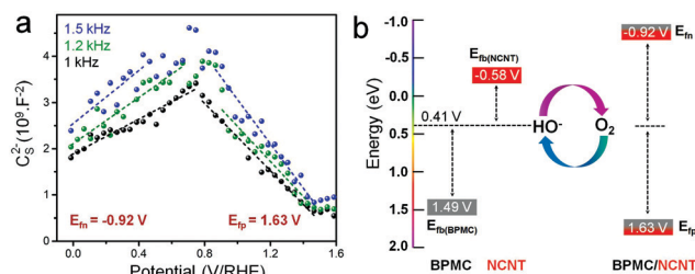
Fig. 2 (a) Mott Schottky plots of BPMC/NCNT-10 at three different frequencies. (b) Schematic diagram of E_{\text{fb}} alignment of BPMC, NCNT and BPMC/NCNT-10 with respect to standard \text{O}_2 electrolysis potential in alkaline medium.
