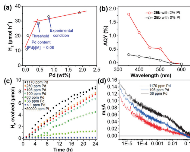
Fig. 15 (a) H 2 evolution of polymer 25b with different residual Pd contents. (b) Apparent quantum yield (AQY) of polymer 25b with 2% and without Pt loading at different wavelengths. (c) H 2 evolution of nanoparticles of polymer 15 with different amounts of Pd or Pt. (d) Transient kinetics of nanoparticles of polymer 15 with different Pd concentrations in a diethylamine/water mixture. Reprinted with permission from ref. 105 and 161. Copyright 2016 American Chemical Society and 2018 Wiley-VCH.
