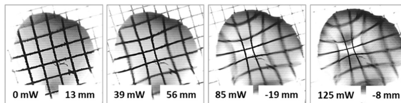
Fig. 7 Images of the test grid obtained with the thermocapillary lens (benzyl alcohol, 0.6 \mu l) at different laser beam powers. 30
