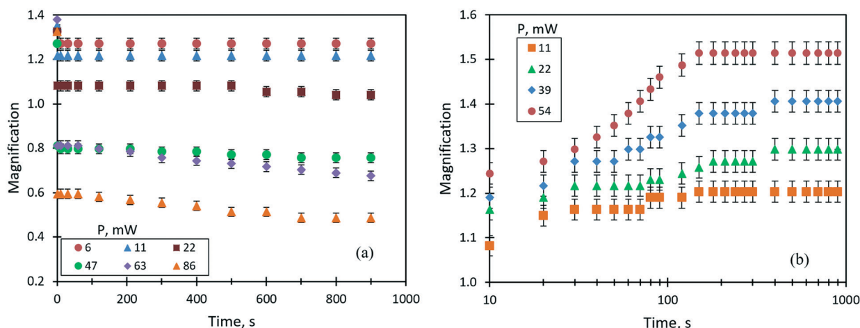
Fig. 8 Evolution of the linear magnification of liquid lenses at different powers of the laser beam: (a) benzyl alcohol (0.6 \mu l), the thermocapillary mechanism; (b) 50% mixture of ethylene glycol and ethyl alcohol (1 \mu l), the solutocapillary mechanism.
