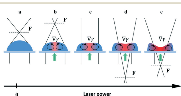
Fig. 2 Schematic illustration of the droplet reshaping by the thermocapillary forces induced with the laser beam. The axis shows the laser power increase. \nabla \gamma is the thermal surface tension gradient along the liquid interface. (a) The initial shape of the droplet (the laser is off); (b) the flattening of the droplet surface – the focal length increases (the laser is on); (c) the droplet with the flat surface – the focal length tends to infinity; (d) and (e) the formation of thermocapillary dimple in the droplet, negative focal length.
