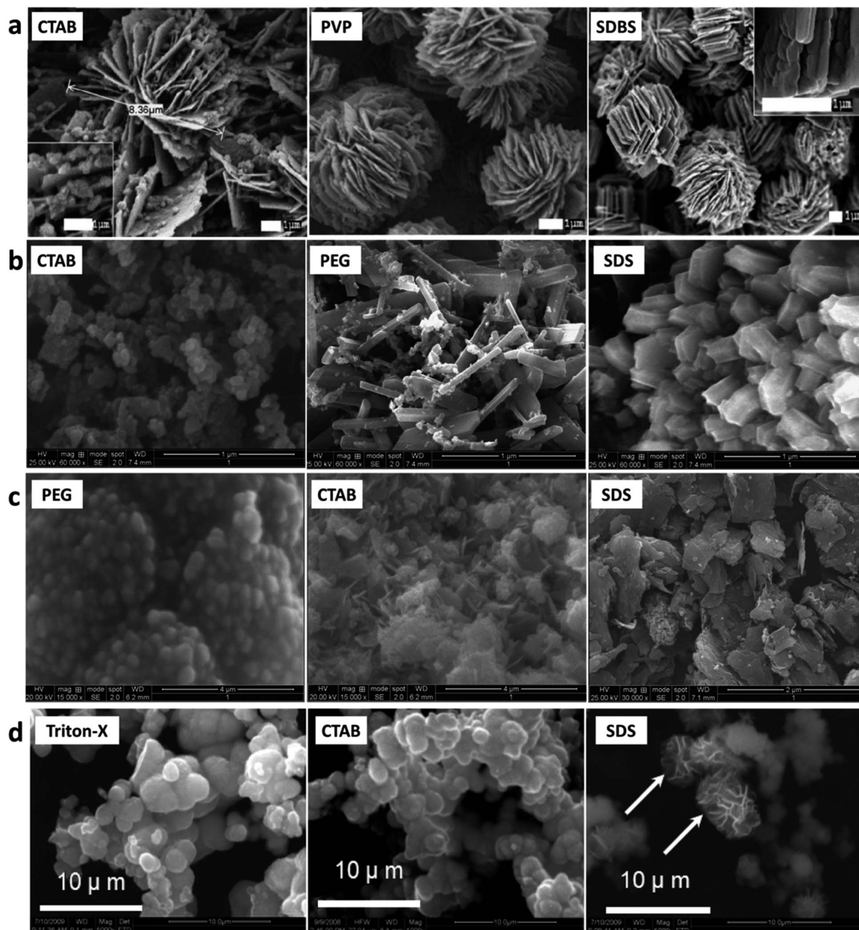
Fig. 6 Diverse morphologies of the same TMOs synthesized using different surfactants. (a) \text{V}_2\text{O}_5 . Reprinted from Hu B., Cheng H., Huang C., Aslam M. K., Liu L., Xu C., Chen P., Yu D. and Chen C., The Controlled Study of Surfactants on the Morphologies of Three-Dimensional Turbine-like \text{V}_2\text{O}_5 for the Application of High-Performance Lithium-Ion Storage, Solid State Ionics , 342 , 115059, Copyright (2019), with permission from Elsevier. (b) \text{NiO} . Reprinted from Rajendran V. and Anandan K., Different Ionic Surfactants Assisted Solvothermal Synthesis of Zero-, Three and One-Dimensional Nickel Oxide Nanostructures and Their Optical Properties, 203–208, Mater. Sci. Semicond. Process. , 38 , Copyright (2015), with permission from Elsevier. (c) \text{Cr}_2\text{O}_3 . Reprinted from Anandan K. and Rajendran V., Sheet, Spherical and Plate-like Chromium Sesquioxide ( \text{Cr}_2\text{O}_3 ) Nanostructures Synthesized via Ionic Surfactants-Assisted Facile Precipitation Method, Mater. Lett. , 146 , 99–102, Copyright (2015), with permission from Elsevier. (d) \text{NiO} . "Reprinted with permission from ref. 197. Copyright (2010) American Chemical Society."
