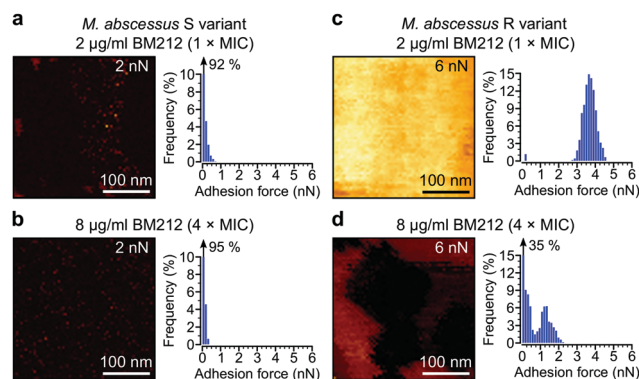
Fig. 5 Inhibiting mycolic acid transport dramatically alters M. abscessus surface hydrophobicity. (a and b) Representative high-magnification adhesion map (300 nm × 300 nm, left) and corresponding histograms of adhesion forces (right) obtained with hydrophobic tips for the M. abscessus S variant treated with BM212 at 1× (a) or 4× its MIC (b). The z-range for each map is indicated in the top right corner. (c and d) Adhesion maps and histograms of the M. abscessus R variant obtained under similar conditions. At least eight cells from two independent experiments per strain and treatment condition showed similar results.
