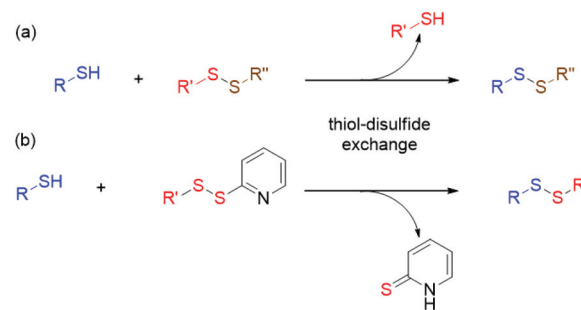
Scheme 2 General representations of (a) thiol–disulfide, and (b) thiol–pyridyl disulfide exchange reactions.
